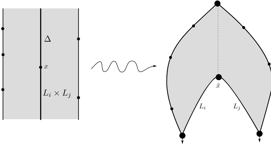
FIGURE 23. The equality between the quilted strip controlling \mathbf{M}_{\Delta, L_i \times L_j}^1 and the first-order map \mathcal{CY}_{L_i, L_j}^{0|1|0} .
