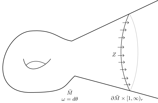
FIGURE 1. A Liouville manifold with cylindrical end.
