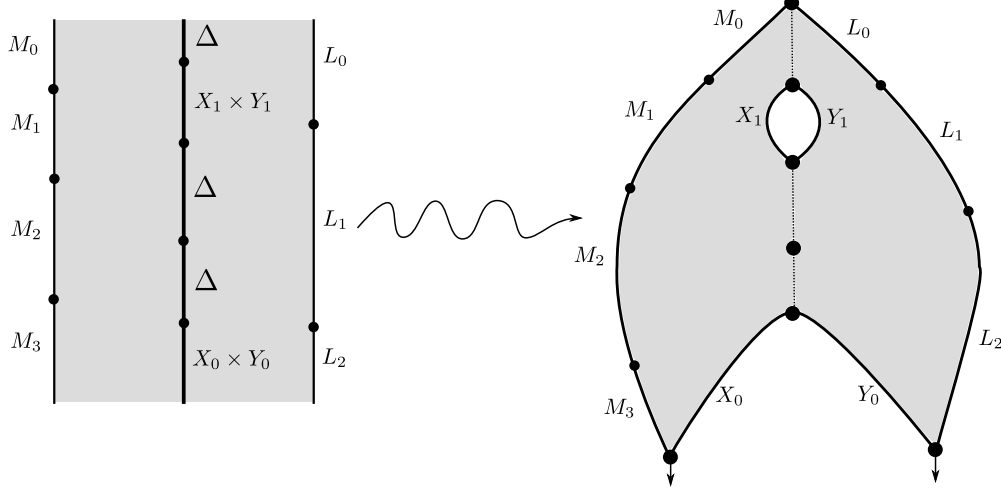
FIGURE 15. An example of the quilt unfolding \Psi_{\hat{L}} .
