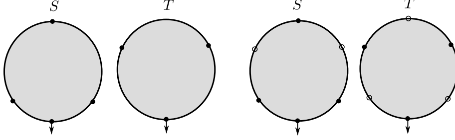
FIGURE 18. An example of the overlay map from {}_0\mathcal{R}_{3,2} to \mathcal{R}_{5,5}^{\{2,4\},\{1,3,5\}} .
