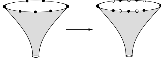
FIGURE 19. The overlay map from \mathfrak{S}, p(\mathfrak{S})\mathcal{R}_{5,4} to \mathfrak{S}', p(\mathfrak{S}')\mathcal{R}_{7,7}^{\{3,5\}, \{2,4,6\}} , where \mathfrak{S} = \{(1,1), (5,4)\} and \mathfrak{S}' = \{(1,1), (7,7)\} . Forgotten points are marked with rings.
